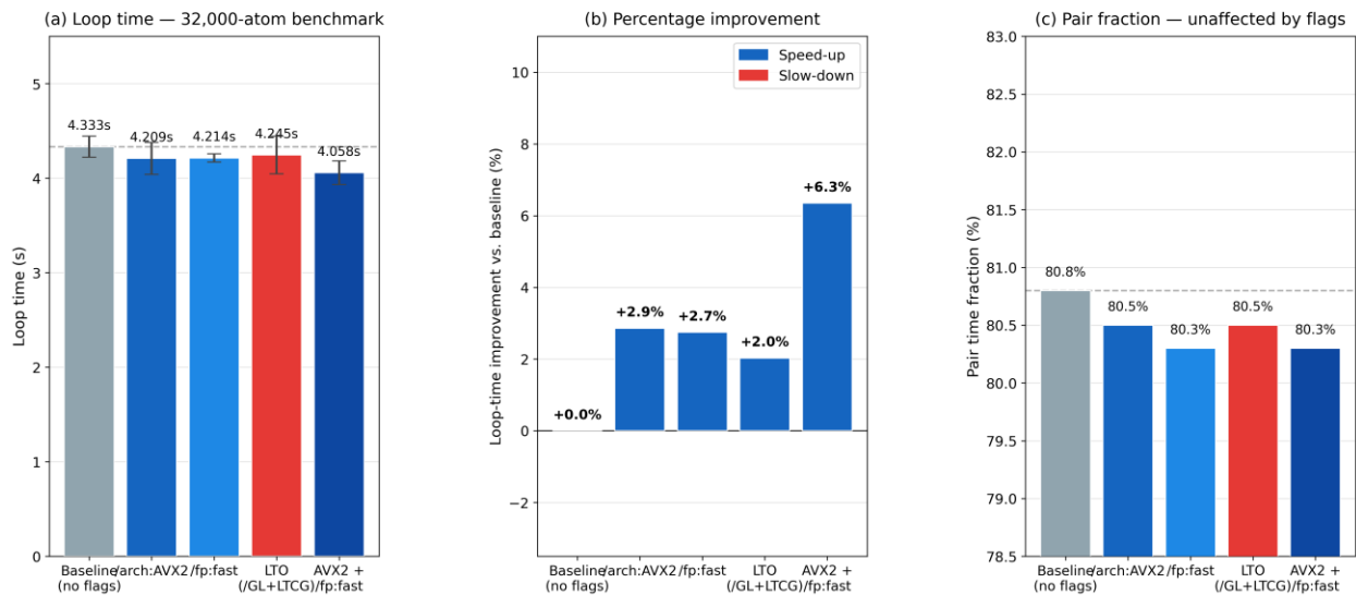
Figure 3: Compiler flag optimization on the 32,000-atom benchmark. (a) Loop time (mean \pm 1 std, N=5 runs) for baseline and four flag configurations. Horizontal dashed line indicates baseline. (b) Percentage improvement in loop time relative to baseline. The AVX2+ /fp:fast combination delivers 6.3% improvement while LTO shows marginal and variable gain. (c) Pair time fraction vs. configuration, confirming that non-pair sections (neighbor, comm) are not adversely affected.
