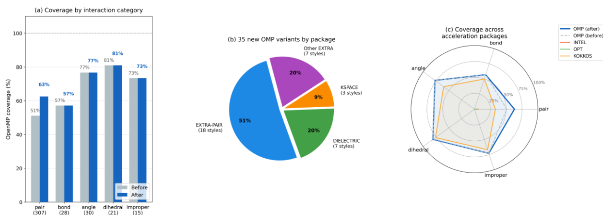
Figure 2: OpenMP acceleration coverage in LAMMPS before and after optimization. (a) Coverage fractions for each interaction category before optimization (grey) and after addition of 35 new pair_style OMP variants (colored). Error bars indicate \pm 1 for single-style uncertainty in manual counting. (b) Breakdown of the 35 new OMP pair variants by source package. (c) Radar chart comparing OMP, INTEL, OPT, and KOKKOS package coverage
