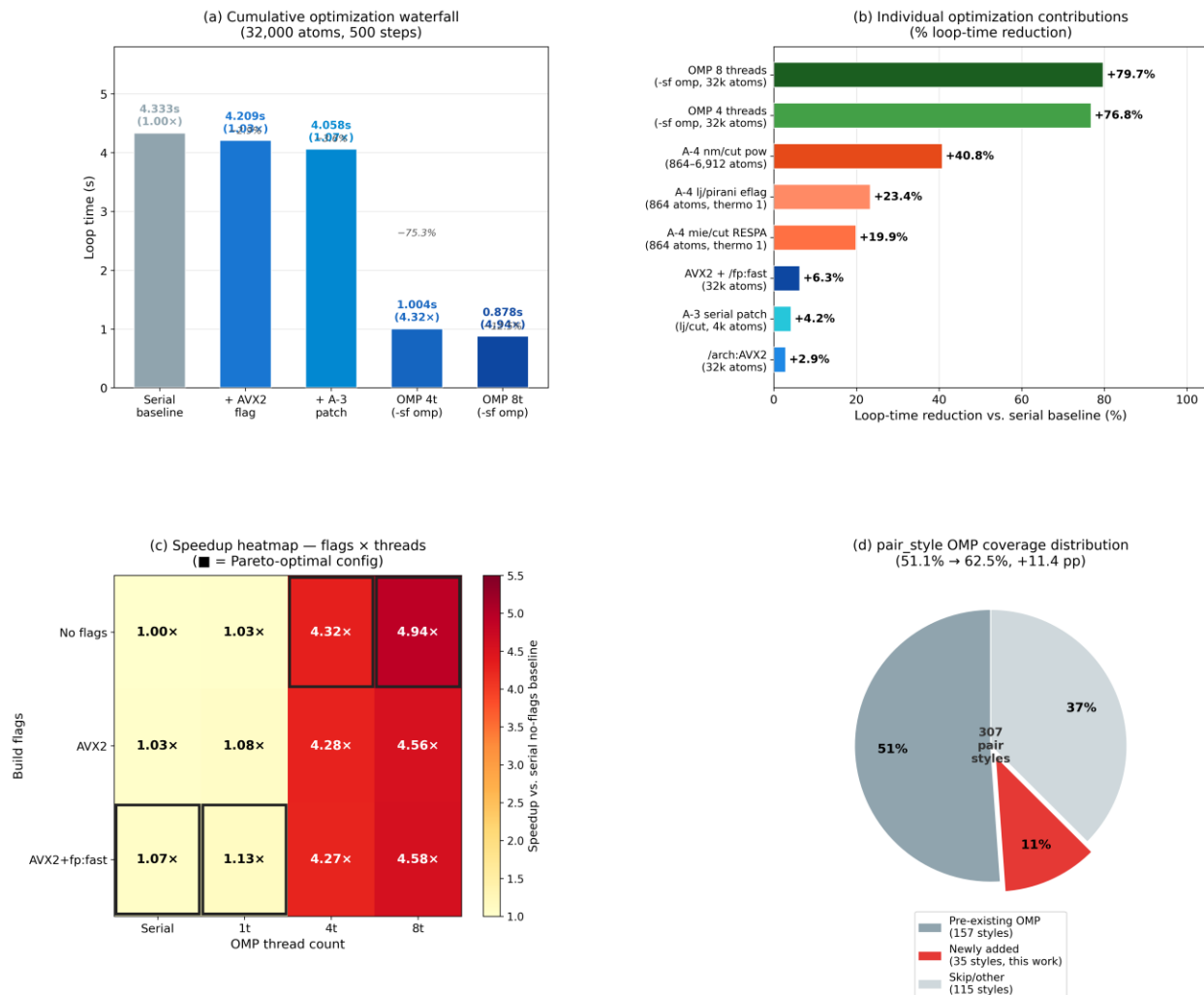
Figure 5: Combined optimization summary. (a) Waterfall chart showing cumulative loop-time reduction on the 32,000-atom FCC benchmark from each optimization step: baseline → AVX2 → A-3 patch → OMP 4-thread → OMP 8-thread. (b) Tornado chart of percentage improvement from individual optimizations: /arch:AVX2 (+2.9%), A-3 serial patch (+4.2%), AVX2+/fp:fast (+6.3%), A-4 mie/cut RESPA (+19.9%), A-4 lj/pirani eflag (+23.4%), A-4 nm/cut pow reduction (+40.8%), OMP 4t (+76.8%), OMP 8t (+79.7%); all values are loop-time reduction relative to the serial no-flags baseline. (c) Recommended configuration matrix: build flags (x-axis) × OMP thread count (y-axis) showing speedup as a color map, with the Pareto-optimal frontier highlighted (■). (d) Impact on OMP pair_style coverage: before (157/307 = 51.1%) and after (192/307 = 62.5%) this work.
