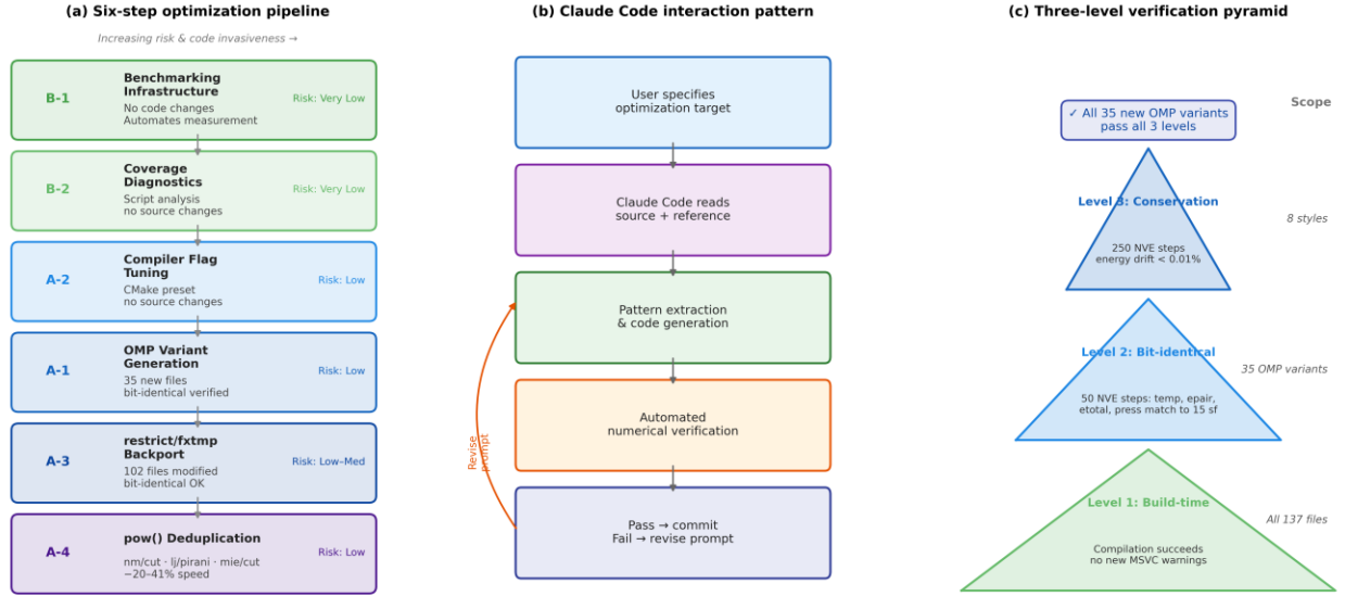
Figure 1: AI-assisted LAMMPS optimization workflow. (a) Six-step optimization pipeline organized by risk and LLM suitability. Risk increases from Step B-1 (no code changes) to Step A-3 (in-place modification of ~102 files). (b) Claude Code interaction pattern: the LLM reads reference implementations, extracts transformation patterns, generates new code, and triggers automated numerical verification. (c) The three-level verification pyramid: build-time (compilation), single-step (bit-identical thermo output), and multi-step (NVE energy conservation).
